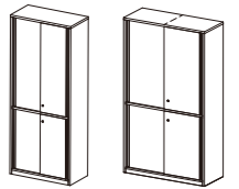
Wooden Sliding Door High Cabinet UL-2007S 700W x 400D x 2000H UL-2008S 800W x 400D x 2000H UL-2009S 900W x 400D x 2000H UL-2010S 1000W x 400D x 2000H UL-2011S 1100W x 400D x 2000H UL-2012S 1200W x 400D x 2000H UL-2013S 1300W x 400D x 2000H
