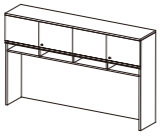
Hutch Cabinet UL-1116WH 1600W x 400D x 1150H UL-1118WH 1800W x 400D x 1150H UL-1120WH 2000W x 400D x 1150H UL-1216WH 1600W x 400D x 1250H UL-1218WH 1800W x 400D x 1250H UL-1220WH 2000W x 400D x 1250H
