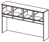
Hutch Cabinet UL-1116GWH 1600W x 400D x 1150H UL-1118GWH 1800W x 400D x 1150H UL-1120GWH 2000W x 400D x 1150H UL-1216GWH 1600W x 400D x 1250H UL-1218GWH 1800W x 400D x 1250H UL-1220GWH 2000W x 400D x 1250H
